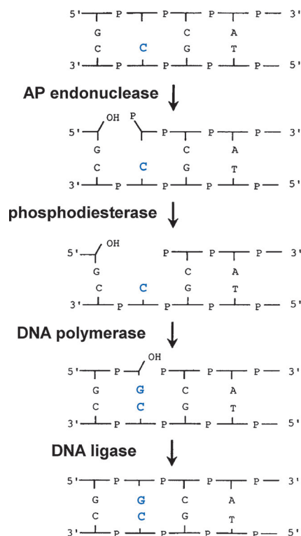
Figure 4. Repair of abasic sites in DNA. Lindahl, Nature , 1993.
