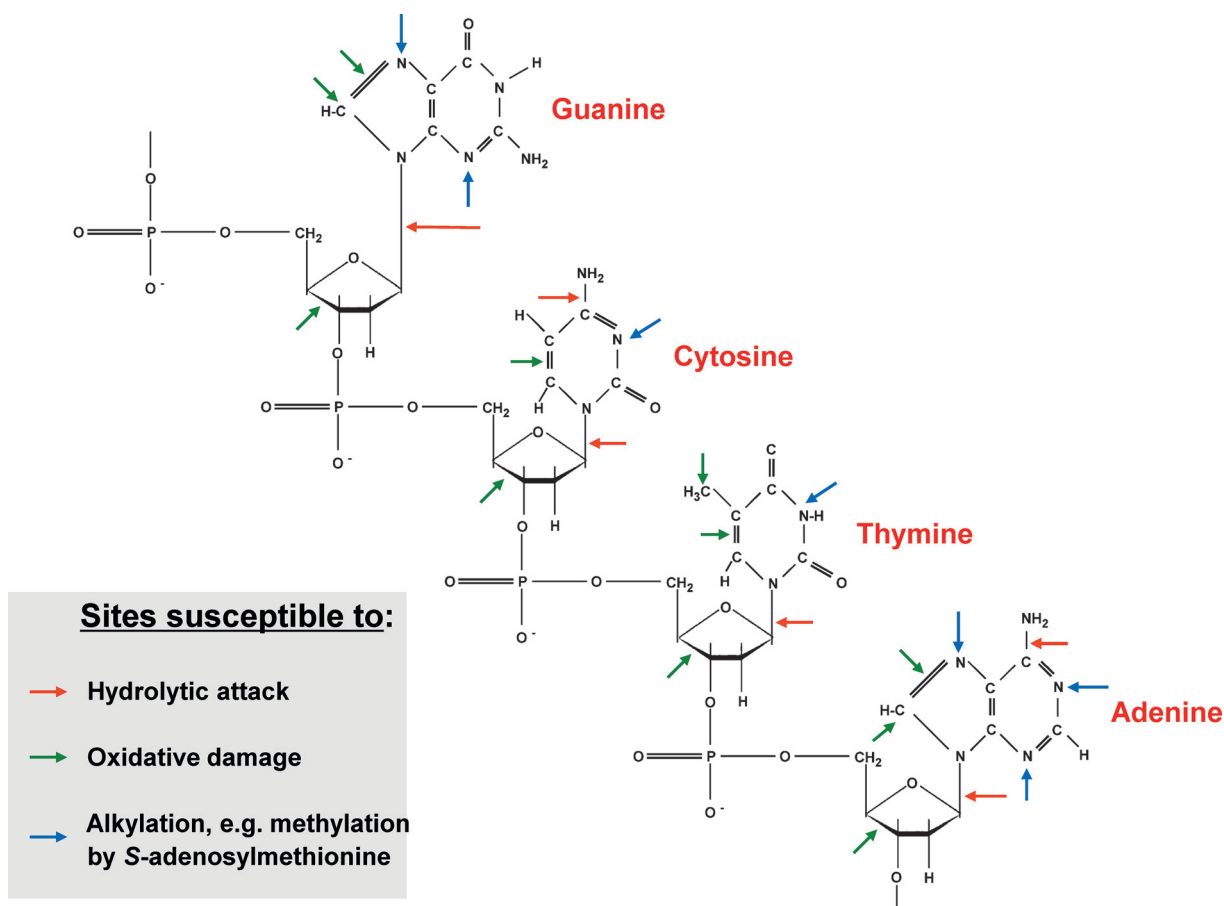
Figure 2. DNA lability (especially depurination). Lindahl, Nature , 1993.
