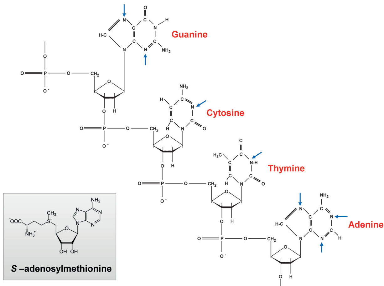
Figure 8. DNA lability: Alkylation. Lindahl, Nature , 1993.
