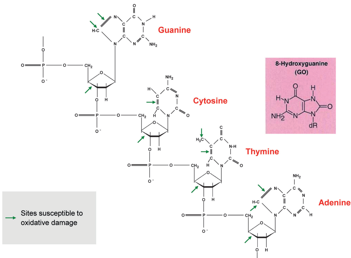
Figure 7. DNA lability: Oxidative damage. Lindahl, Nature , 1993.
